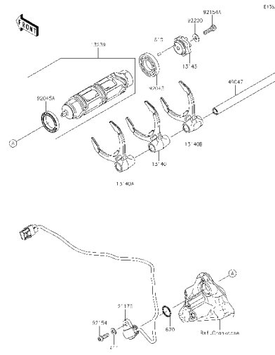
C-4 Gear Change Drum/Shift Fork(s)
