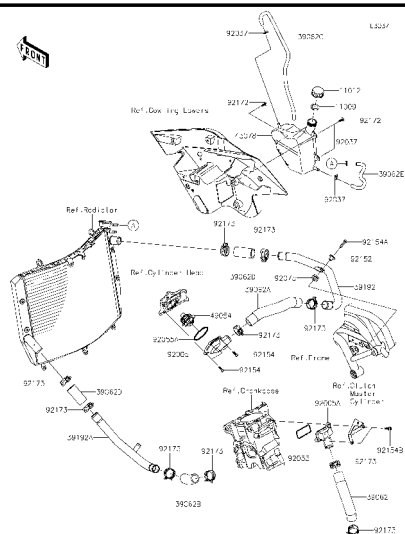
D-12 Water Pipe
