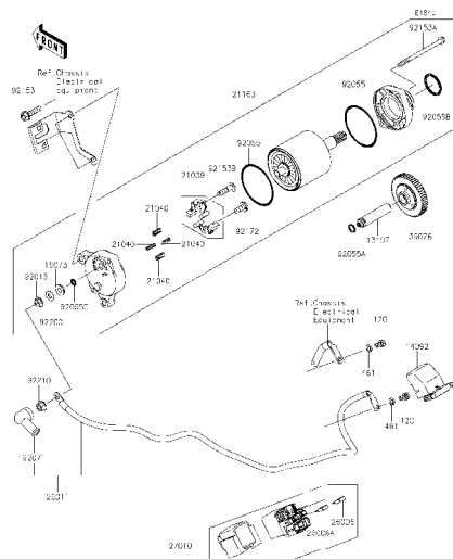
D-9 Starter Motor
