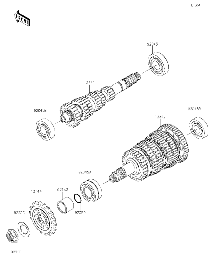
C-3 Transmission
