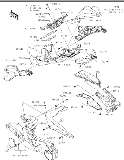
E-9 Rear Fender(s)
