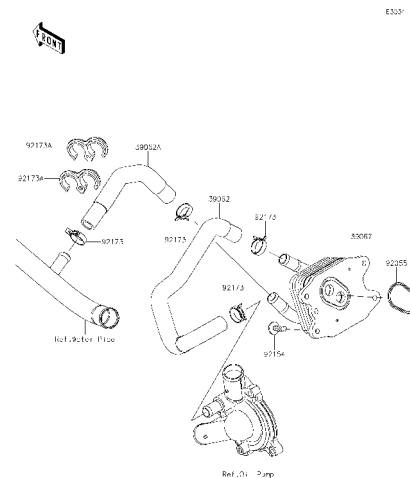
D-11 Oil Cooler
