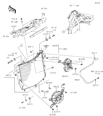
D-10 Radiator
