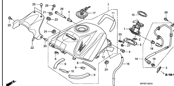
FUEL TANK (CBR125RW7/RW9/RWA)
