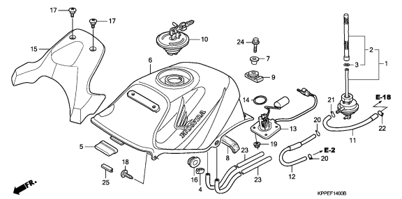
FUEL TANK (CBR125R/RS/RW5/RW6/RW8)
