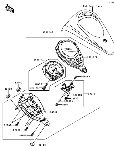
F-13 Meter(s)
