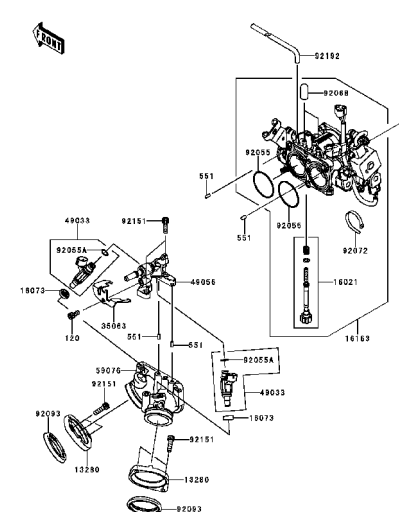
C-8 Throttle
