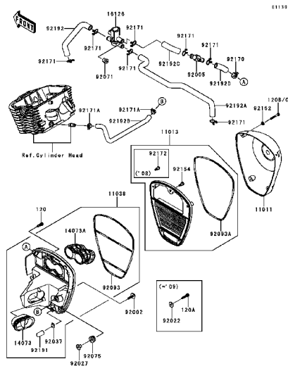
B-6 Air Cleaner
