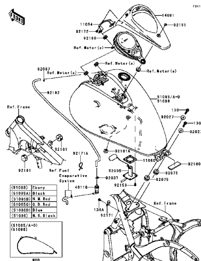
F-10 Fuel Tank(1/2)
