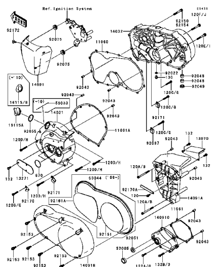
C-6 Engine Cover(s)(1/2)
