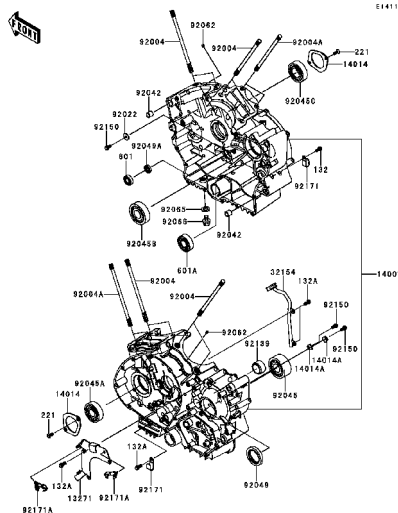
C-4 Crankcase
