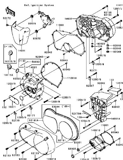
C-7 Engine Cover(s)(2/2)
