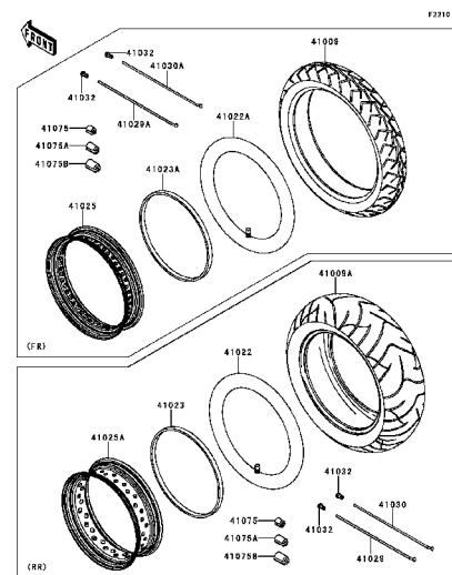
E-12 Tires
