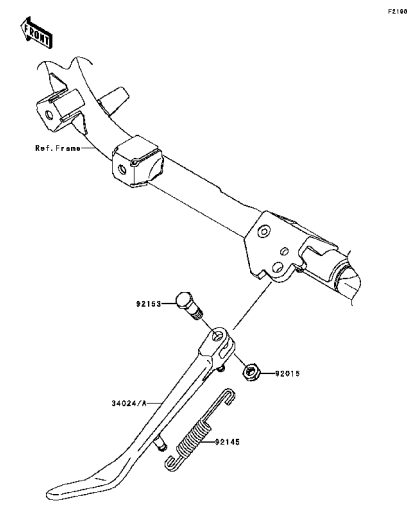
E-11 Stand(s)
