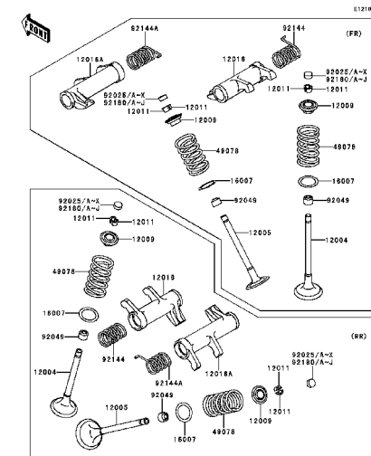
B-8 Valve(s)(1/2)
