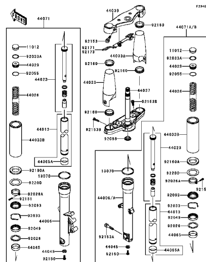
F-9 Front Fork
