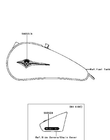
G-11 Decals(B8F/B9F)
