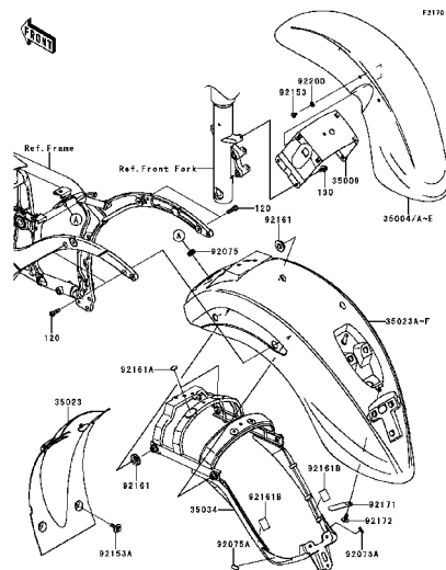
E-9 Fenders(1/2)
