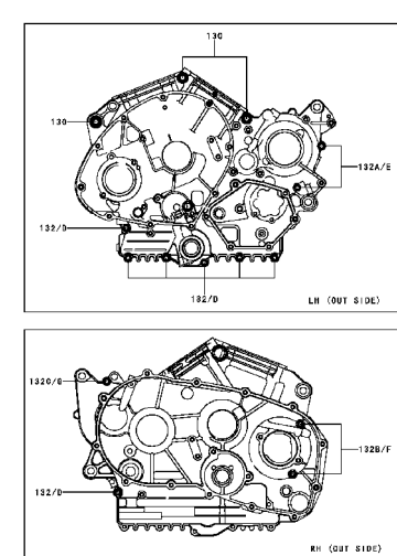
C-5 Crankcase Bolt Pattern
