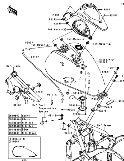
F-11 Fuel Tank(2/2)
