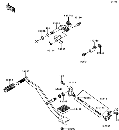
C-3 Gear Change Mechanism
