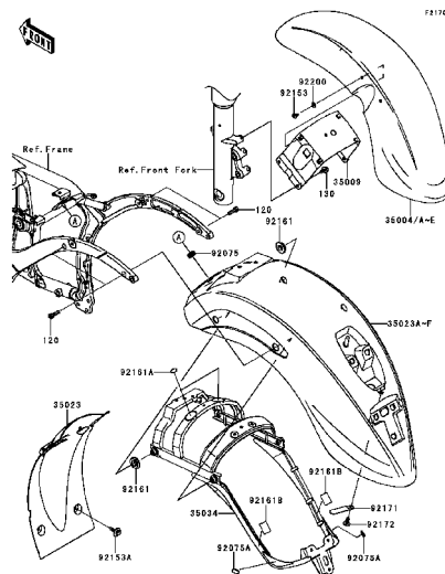
E-10 Fenders(2/2)
